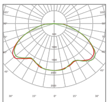
25W/40W/60W beam angle
