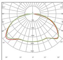
80W/100W beam angle
